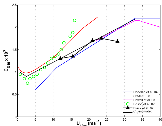
Fig. 16. Drag coefficient estimates as a function of the 10 m neutral wind from the several recent studies shown in the legend. The black solid line shows the C_D obtained from them for this study.
