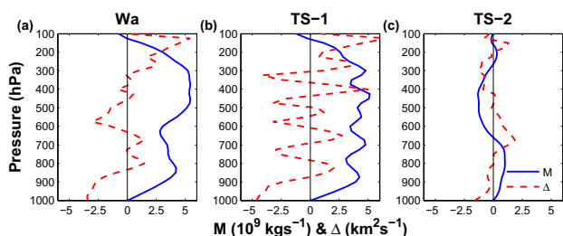
Fig. 10. Vertical profiles of horizontal ( \Delta , red dashed line) and vertical ( M , blue solid line) mass fluxes for tropical storm Eugene at (a) the tropical wave time (Wa), (b) the first tropical storm time (TS-1) and (c) the second tropical storm time (TS-2), before it decayed back to tropical depression stage.
