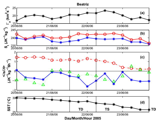
Fig. 13. Same as Fig. 11 but for tropical storm Beatriz. Vertical solid lines delimit the tropical depression (TD) and tropical storm (TS) stages.
