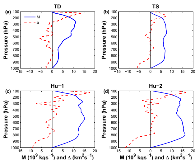
Fig. 8. Vertical profiles of horizontal ( \Delta , red dashed line) and vertical ( M , blue solid line) mass fluxes for hurricane Dennis at (a) the tropical depression time (TD), (b) the tropical storm time (TS), (c) the first hurricane time (Hu-1) and (d) the second hurricane time (Hu-2) analyzed.
