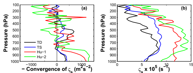
Fig. 7. Vertical profiles of (a) minus the convergence of absolute vorticity and (b) absolute vorticity at the cyclone's boundary averaged over the 4^\circ \times 4^\circ area at four times during hurricane Dennis' life cycle. Tropical depression time (TD, black line), tropical storm time (TS, blue line), first hurricane time (Hu-1, red line) and second hurricane time (Hu-2, green line).
