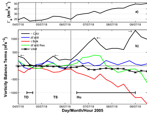
Fig. 3. Hurricane Dennis. (a) Time evolution of the absolute circulation averaged in the layer 1000–900 hPa. (b) Terms in the balance of Eq. (6) averaged in the layer 1000–900 hPa. The black line represents minus the convergence of absolute vorticity ( -CAV ), line with crosses (vertical advection of momentum, VAM), blue line ( \Gamma_a tendency), red line (bulk friction term, \tau Bulk) and green line (residual \Gamma_a tendency). Vertical solid lines delimit the tropical depression (TD), tropical storm (TS) and hurricane (Hu) stages as determined by the NHC. Periods when Dennis made landfall are indicated by horizontal bars. Arrows indicate certain times that will be discussed in the text and in Figs. 7 and 8.
