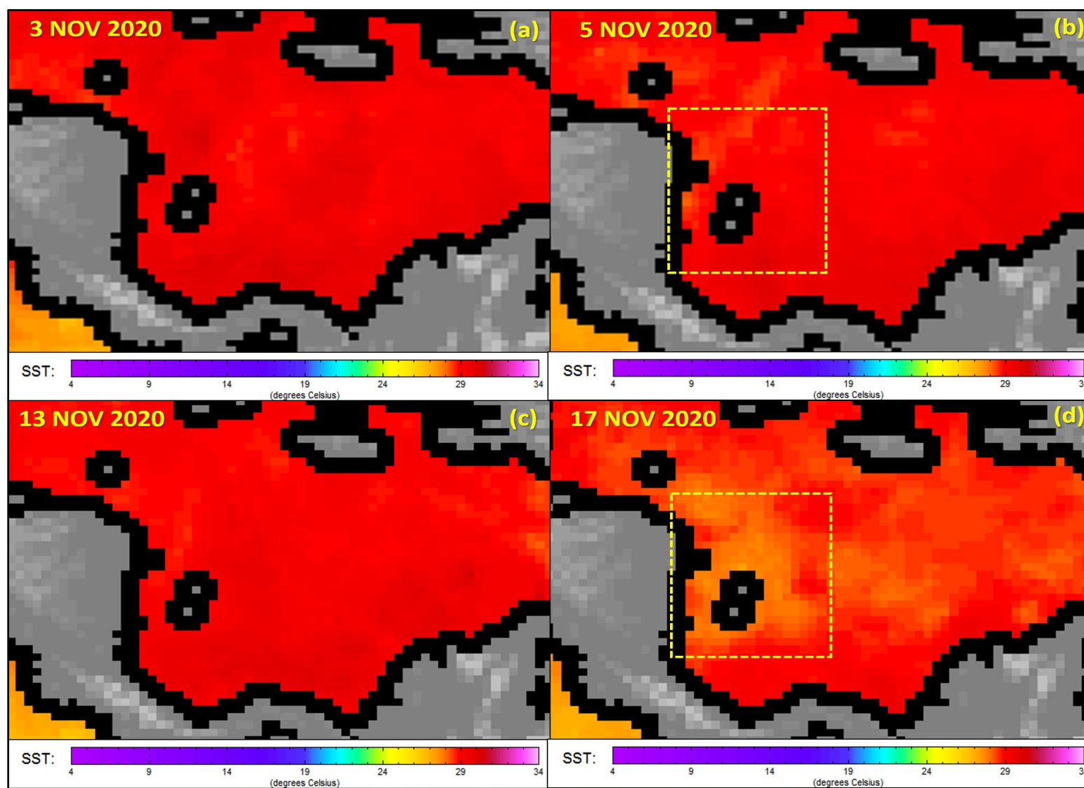
Figure 5. Sea-surface temperature (°C) analyses for Hurricane Eta on 3 November before landfall (a) in Nicaragua and on 5 November 2020 after landfall (b), and for Hurricane Iota on 13 November before landfall (c) in Nicaragua and on 17 November 2020 after landfall (d). The yellow-dashed rectangle indicates area of affected by both Eta and Iota; note area of significant cooling caused by upwelling generated by Hurricane Iota on 17 November. Images courtesy of Remote Sensing Systems, Santa Rosa, CA.
