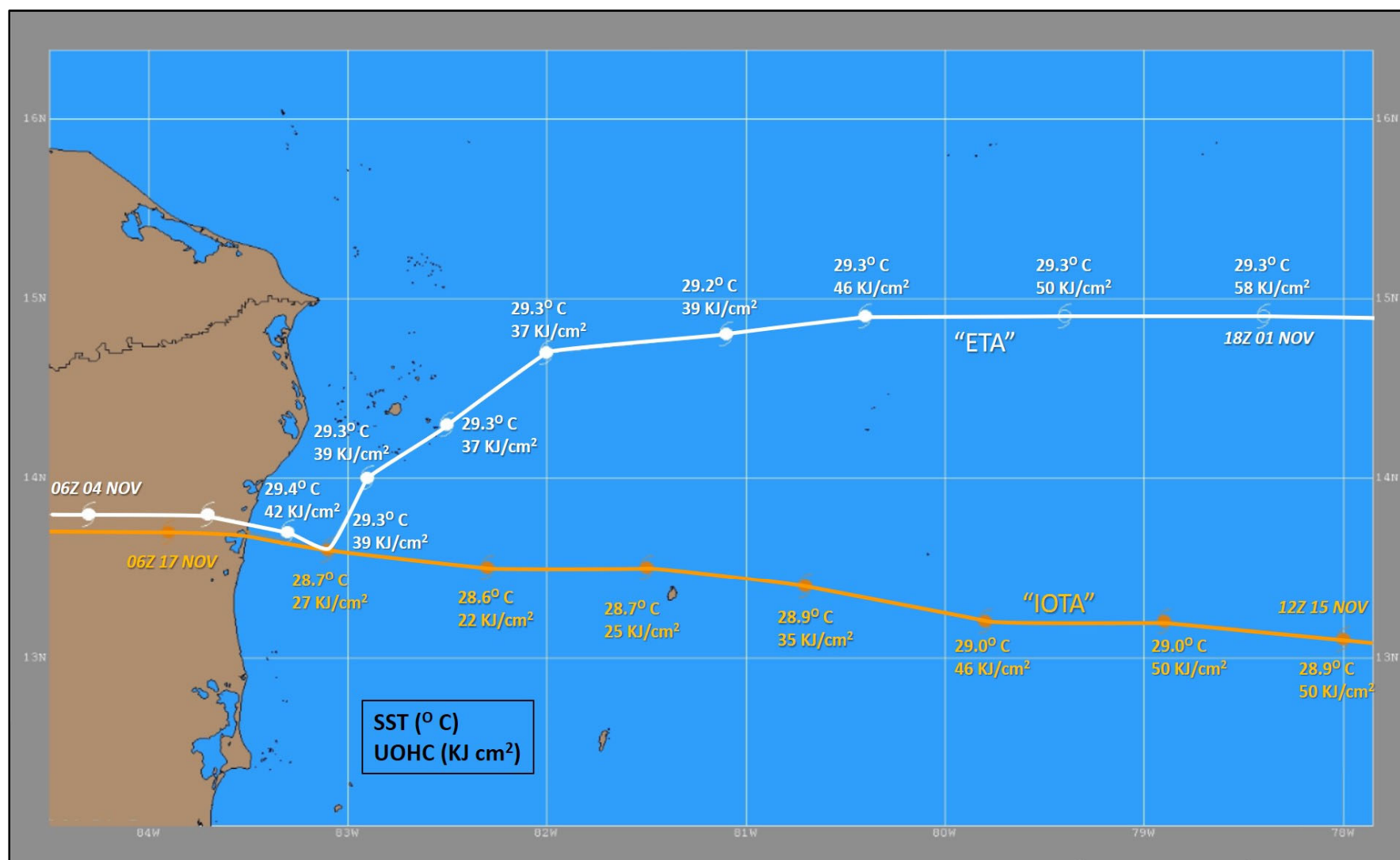
Figure 6. Plots of the ‘best tracks’ for Hurricane Eta, 1–4 November 2020, and Hurricane Iota, 15–17 November 2020. Sea-surface temperatures (SST °C) and Upper-Ocean Heat Content (UOHC KJ cm -2 ) values are superimposed along the tracks at the respective 6-h synoptic times. The southern portion of Eta’s circulation generated mixing and upwelling around Providencia as indicated by the slightly lower SSTs and by the 30% lower UOHC values along Iota’s track.
