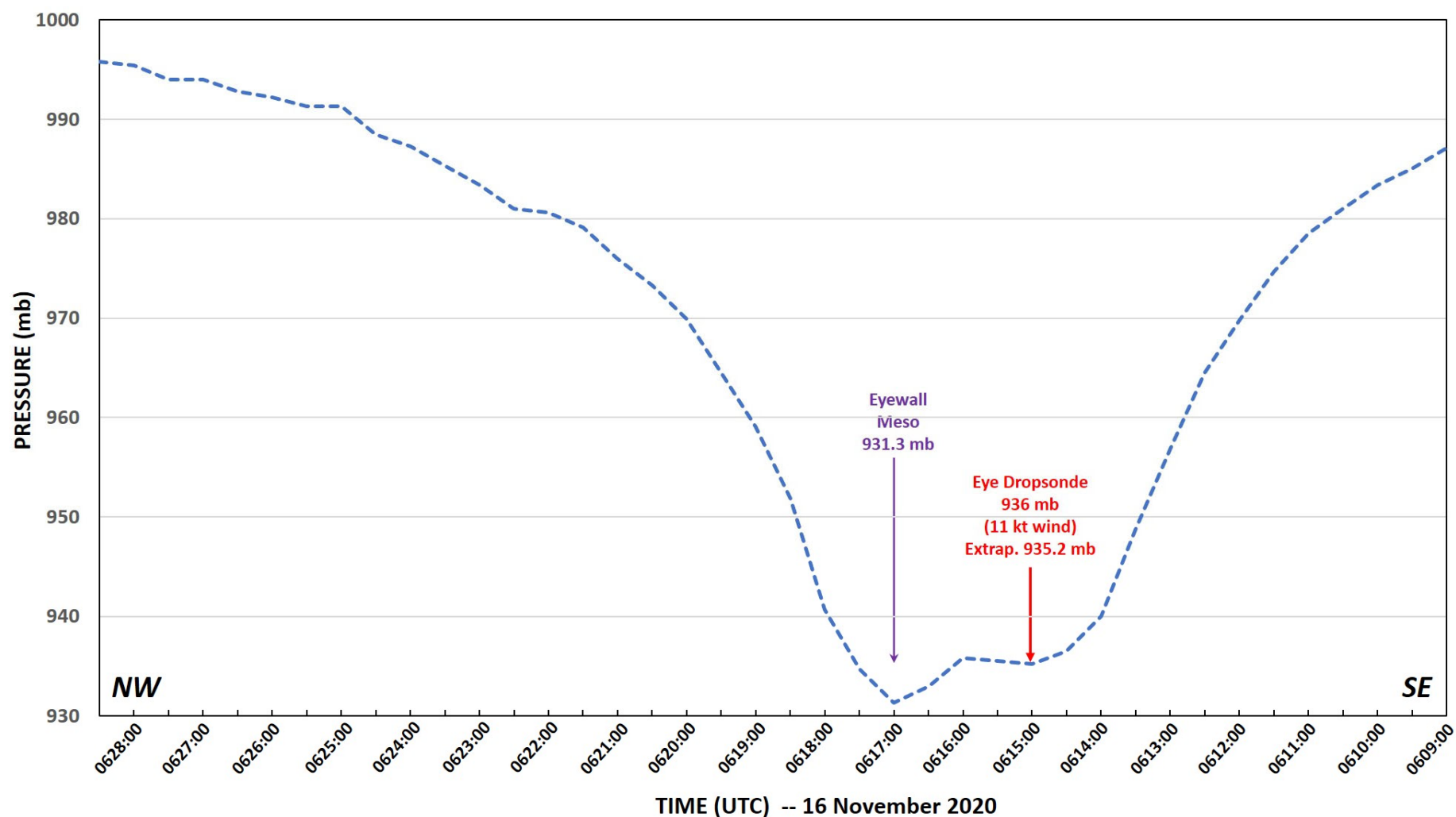
Figure 8b. Aircraft-extrapolated surface pressure plot from 0609:00 UTC to 0628:30 UTC 16 November 2020 (in 30-second time intervals) along flight track shown in Figure 8a. Time increases from right to left to coincide with the southeast-to-northwest (SE-NW) track of the reconnaissance aircraft. The central pressure in the eye as measured by a dropwindsonde was estimated to be 935 mb based on a pressure measurement of 936 mb and an associated 11-kt surface wind, which correlates with the 935.2-mb aircraft-extrapolated surface pressure at 0615:00 UTC. An eyewall mesovortex associated with a pressure perturbation of approximately -4 mb was located northwest of the center of the eye at 0617:00 UTC.
