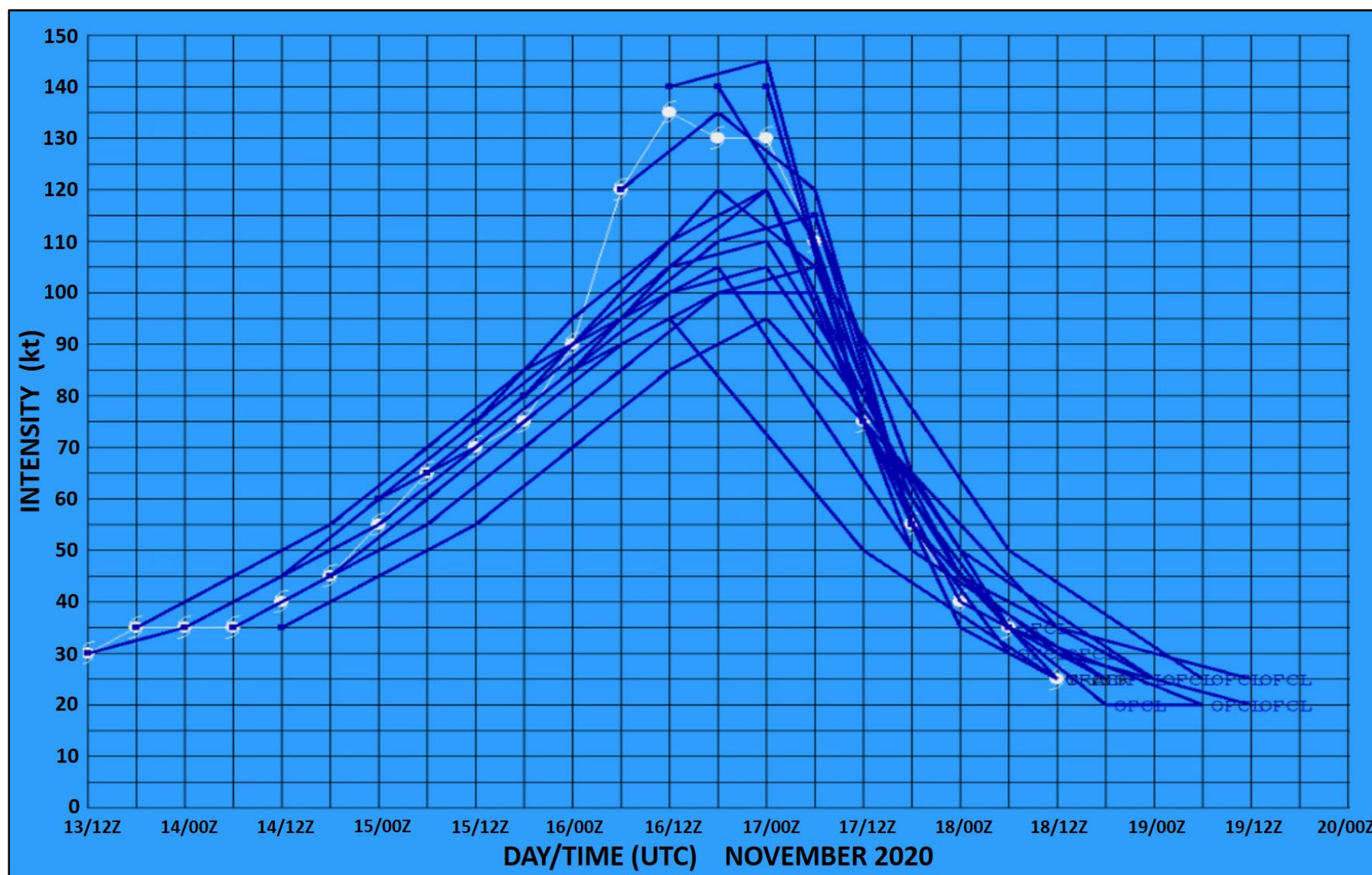
Figure 25. Plot of NHC official intensity forecasts (OFCL, kt) during the period 1200 UTC 13 November to 0600 UTC 18 November 2020. Solid white line indicates the 'best track' intensity estimate (kt) plotted at 6-h forecast intervals (white symbols).
