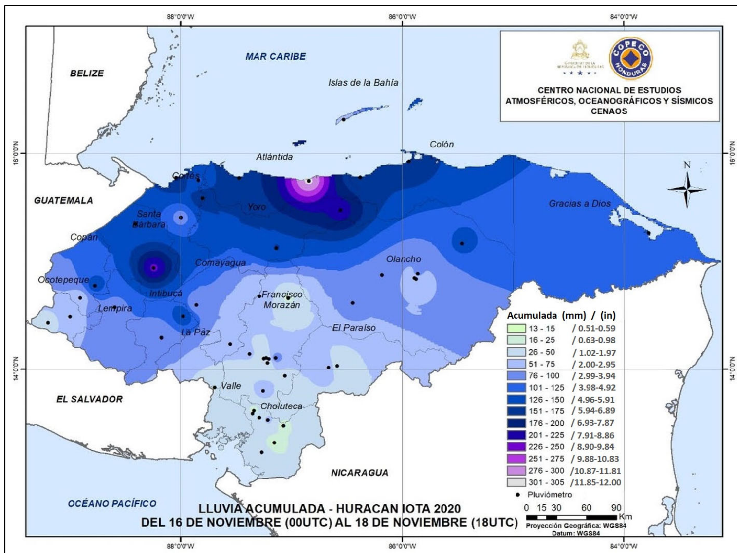
Figure 12. Honduras rainfall totals associated with Hurricane Iota during the period 16–18 November 2020. Graphic courtesy of Centro de Estudios Atmosféricos, Oceanográficos y Sísmicos/CENAOS (Honduras Center for Atmospheric, Oceanographic and Seismic Studies).
