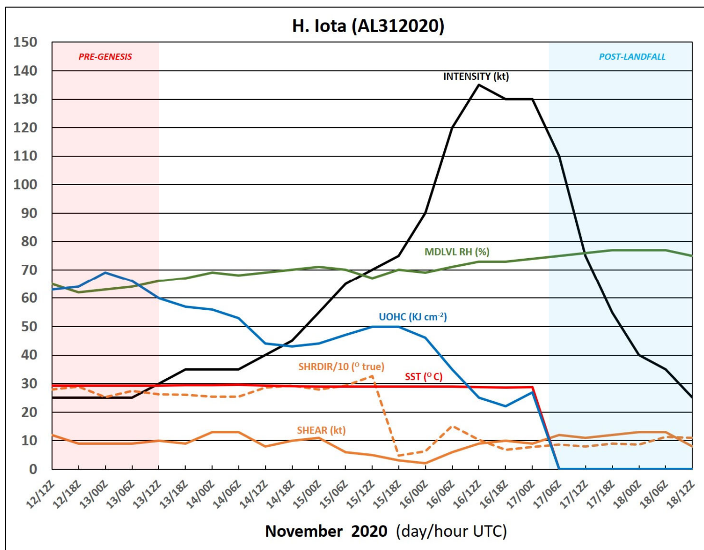
Figure 4. Graph of the INTENSITY (kt) versus GFS-based SHIPS model parameters for Hurricane Iota during the period 12–18 November 2020. SHEAR is 850–200-mb vertical wind shear (kt); SHRDIR/10 is the actual shear direction (dashed line; degrees true) divided by 10; SST is sea-surface temperature (°C); UOHC is upper ocean heat content (KJ cm -2 ); MDLVL RH is 700–500-mb average relative humidity (%). Light-red shaded region represents the pre-genesis period (left) and the light-blue shaded region represents the post-landfall period (right).
