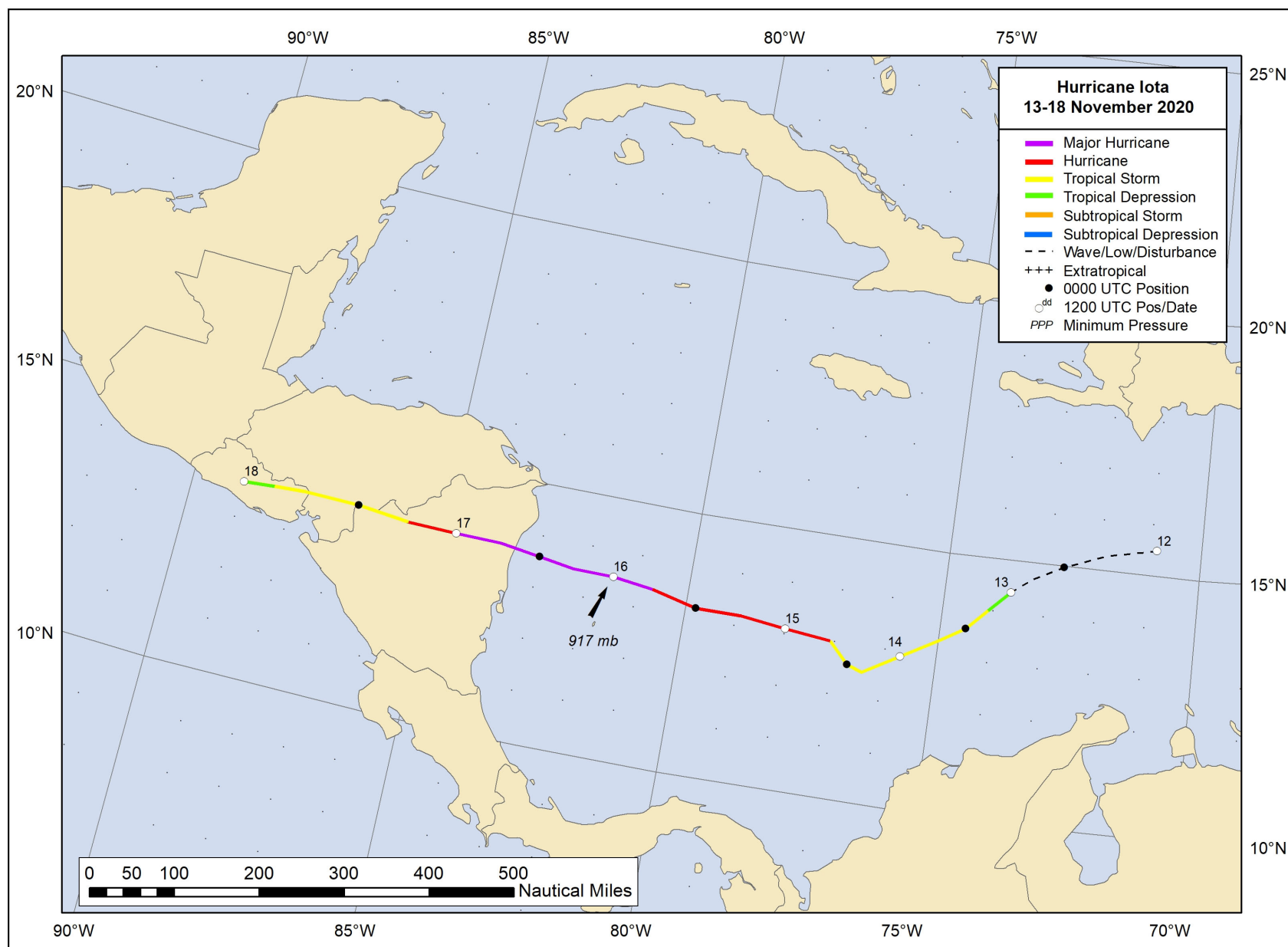
Figure 1. Best track positions for Hurricane Iota, 13–18 November 2020.
