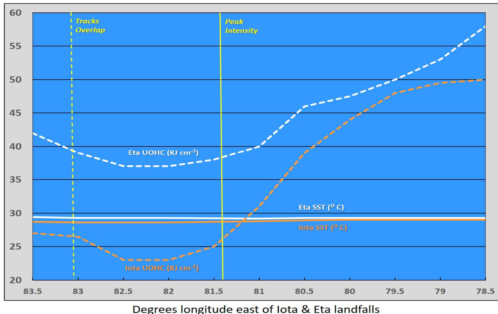
Figure 7. Graphs of the Sea-Surface Temperatures (SST °C) and Upper-Ocean Heat Content (UOHC KJ cm-2) values for Hurricane Eta and Hurricane Iota contained in Figure 7. Data values are plotted along the longitudes east of the landfall longitude (approx. 83.5° W) for each hurricane. Solid-yellow line indicates longitude of Iota's peak intensity and dashed-yellow line indicates the longitude where the tracks of Hurricanes Iota and Eta overlapped leading up to the two landfalls along ~83.5W longitude.
