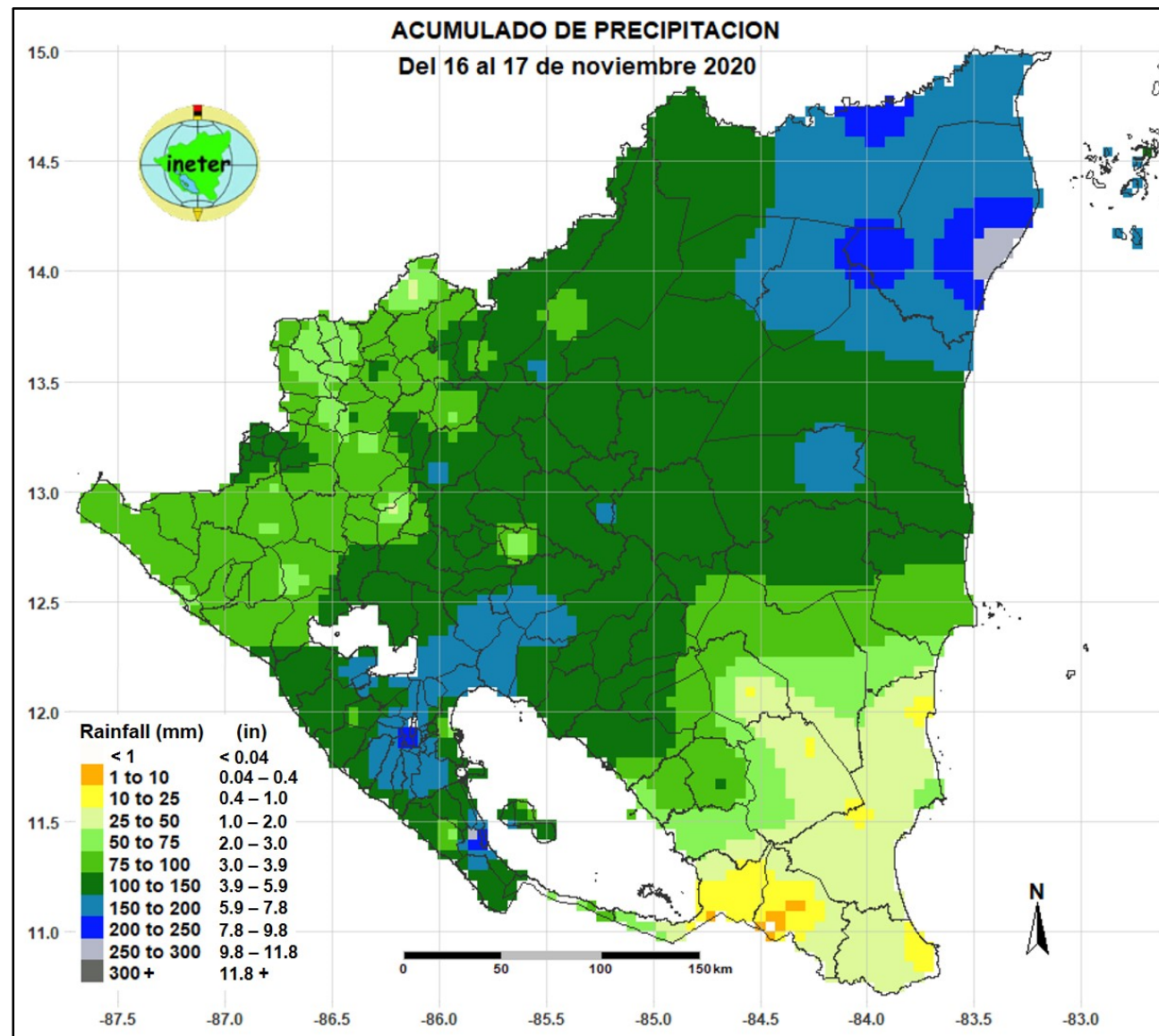
Figure 11. Nicaragua rainfall totals associated with Hurricane Iota during the period 16-17 November 2020. Graphic courtesy of Instituto Nicaraguense de Estudios Territoriales/INETER (Nicaraguan Institute of Territorial Studies).
