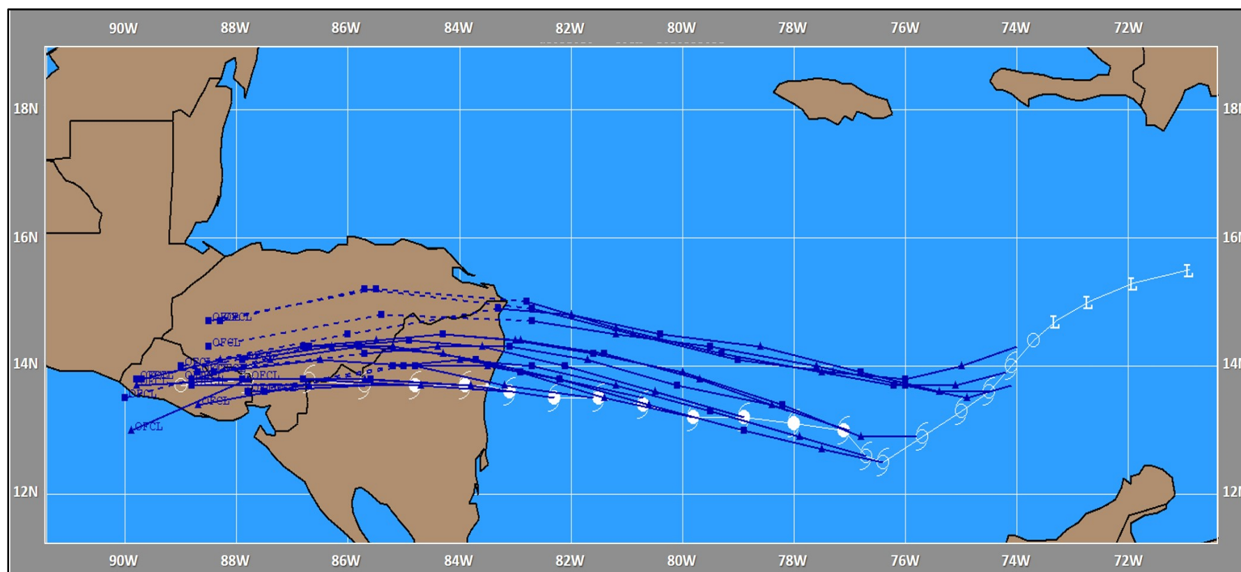
Figure 24. Plot of NHC official 120-h track forecasts (OFCL) during the period 1200 UTC 13 November to 0600 UTC 18 November 2020 (dark blue lines). Solid white line indicates the 'best track', with position estimates at 6-h intervals (white symbols) from 1200 UTC 12 November to 1200 UTC 18 November. The "L" symbols indicate pre-genesis positions.
