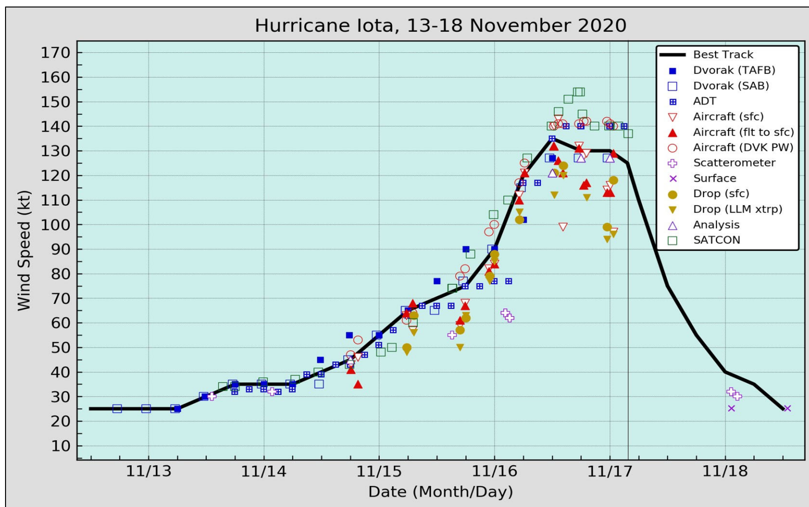
Figure 2. Selected wind observations and best track maximum sustained surface wind speed curve for Hurricane Iota, 13–18 November 2020. Aircraft observations have been adjusted for elevation using 90%, 80%, and 80% adjustment factors for observations from 700 mb, 850 mb, and 1500 ft, respectively. Dropwindsonde observations include actual 10 m winds (sfc), as well as surface estimates derived from the mean wind over the lowest 150 m of the wind sounding (LLM). Advanced Dvorak Technique estimates represent the Current Intensity at the nominal observation time. SATCON intensity estimates are from the Cooperative Institute for Meteorological Satellite Studies. Dashed vertical lines correspond to 0000 UTC. Solid vertical line indicates landfall.
