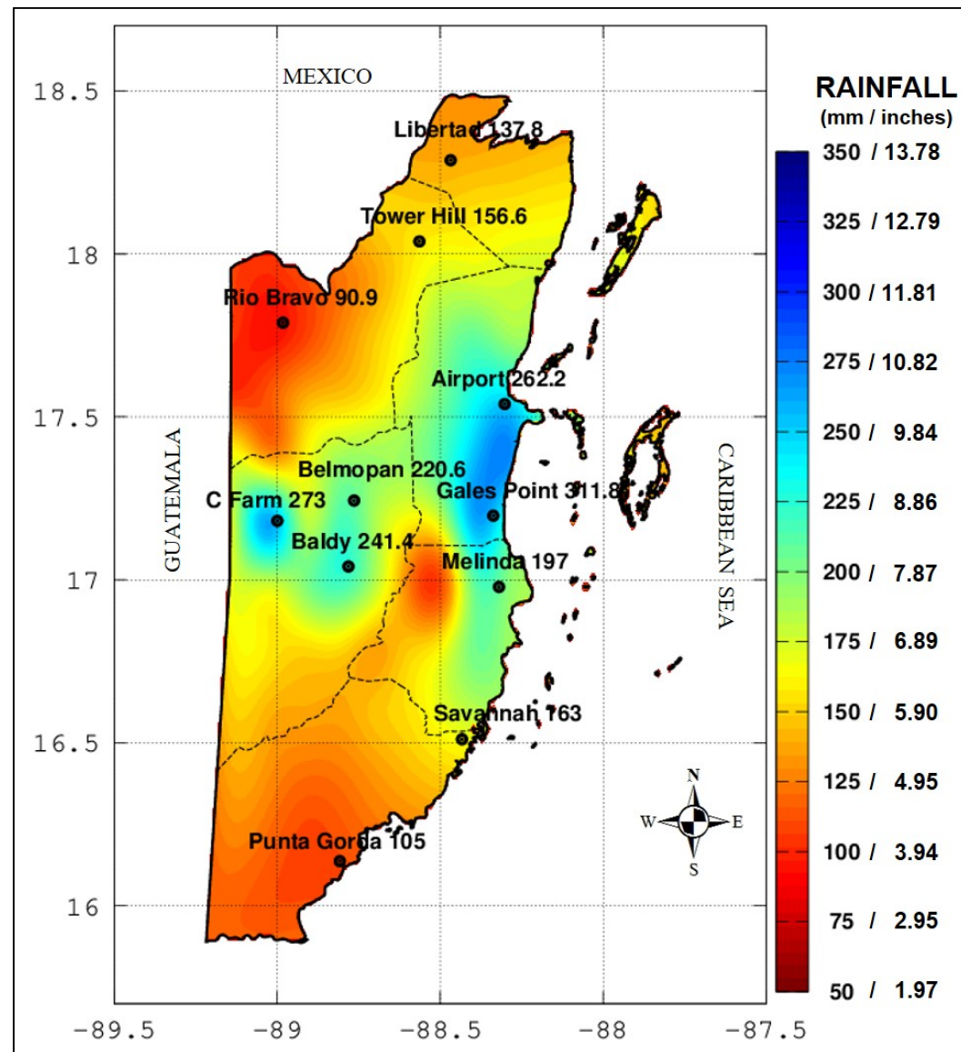
Figure 13. Belize rainfall totals (mm/inches) associated with Hurricane Iota during the period 16–20 November 2020. Graphic courtesy of National Meteorological Service of Belize.
