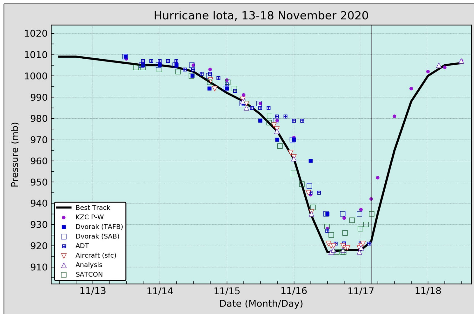
Figure 3. Selected pressure observations and best track minimum central pressure curve for Hurricane Iota, 13–18 November 2020. Advanced Dvorak Technique estimates represent the Current Intensity at the nominal observation time. SATCON intensity estimates are from the Cooperative Institute for Meteorological Satellite Studies. KZC P-W refers to pressure estimates derived using the Knaff-Zehr-Courtney pressure-wind relationship. Dashed vertical lines correspond to 0000 UTC. Solid vertical line indicates landfall.
