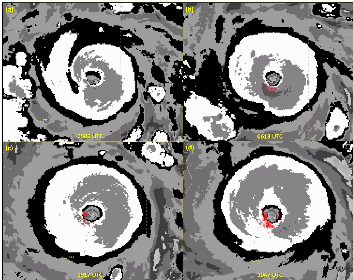
Figure 10. GOES-16 infrared satellite imagery with superimposed 5-minute lightning data (red X's and circles) during Hurricane Iota's rapid intensification (RI) period on 16 November: (a) 0506 UTC, (b) 0618 UTC, (c) 0917 UTC, and (d) 1047 UTC. Lightning began about 0500 UTC in the southwestern quadrant of Iota's eyewall and persisted in that quadrant until RI ended around 1200 UTC later that day.
