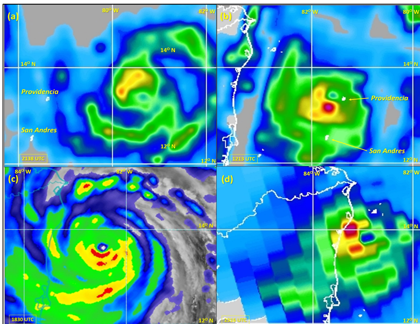
Figure 9. Passive microwave satellite imagery showing the evolution of Hurricane Iota's asymmetrical inner-core convection: (a) 2138 UTC 15 November SSMI/S Rain Rate product showing rainfall rates of about 1.0 in \text{hr}^{-1} in the band located in the northern semicircle; (b) 1213 UTC 16 November SSMI/S Rain Rate product with rainfall rates of >1.4 inch \text{hr}^{-1} in the band in the southern semicircle; (c) 1830 UTC 16 November AMSR-2 89 GHz PCT image showing persistent, intense convection in the southern semicircle; (d) 2316 UTC 16 November AMSU Rain Rate product showing intense convection southwest and west of the eye that contained rainfall rates of >1.4 inch \text{hr}^{-1} along the coast of Nicaragua just east of Puerto Cabezas.
