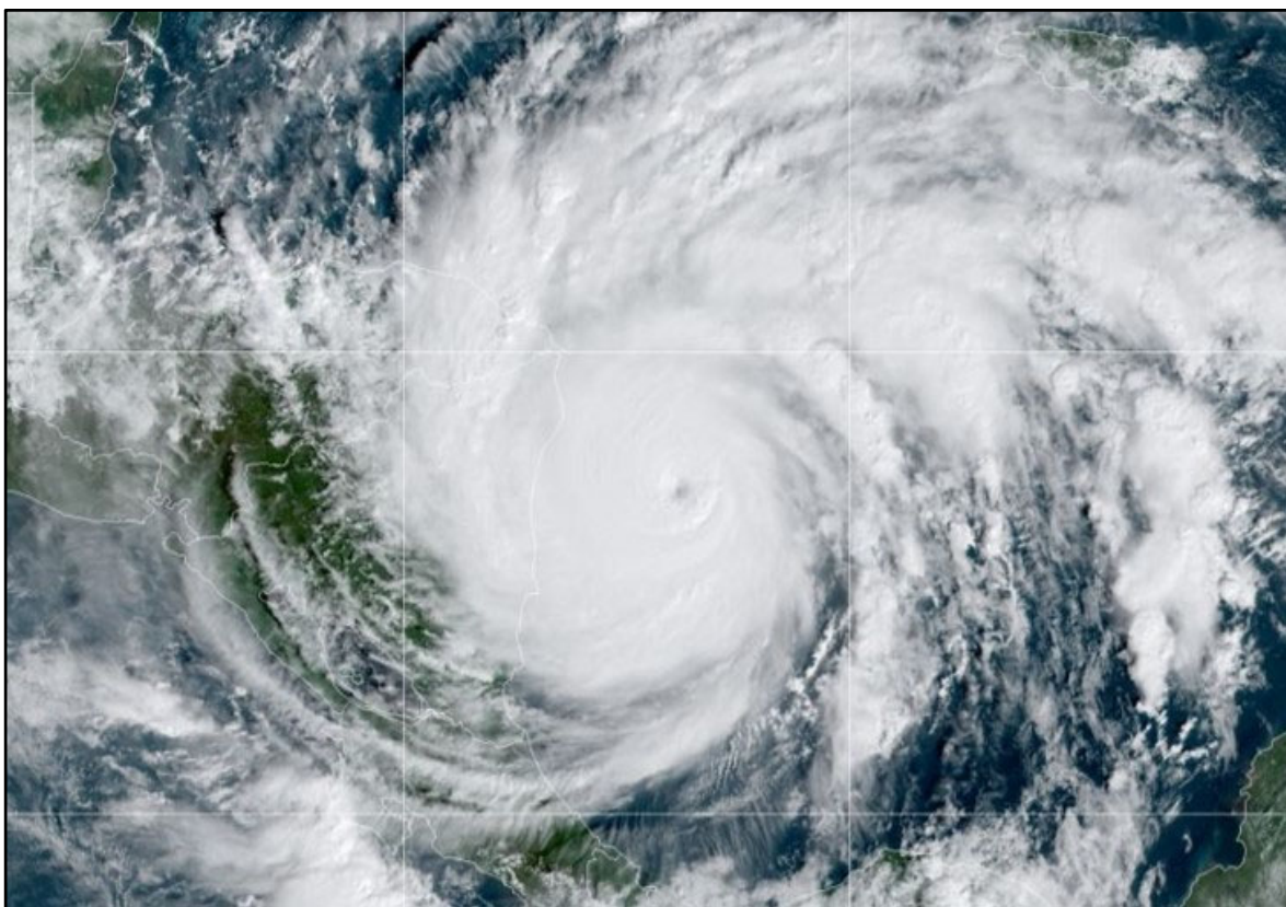
GOES-16 TRUE COLOR VISIBLE SATELLITE IMAGE OF IOTA WHEN IT WAS A STRONG CATEGORY 4 HURRICANE APPROACHING NORTHEASTERN NICARAGUA AT 1430 UTC 16 NOVEMBER 2020. IMAGE COURTESY NOAA/NESDIS/STAR.
